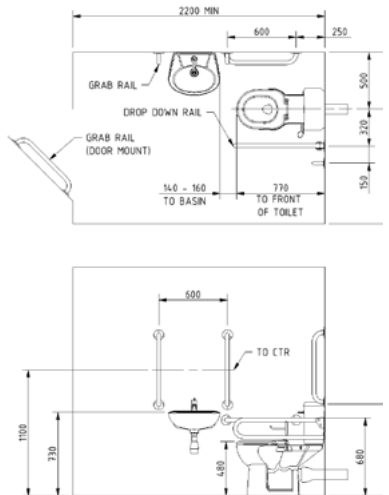
Dimensions (mm)
