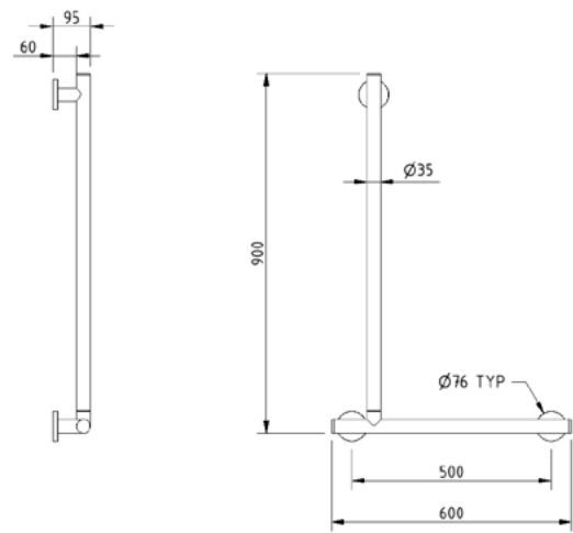
RIGHT-HAND ORIENTATION SHOWN, RAIL CAN ALSO BE SETUP FOR LEFT-HAND ORIENTATION.
