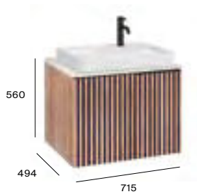
715mm base unit and countertop with one soft-close drawer
