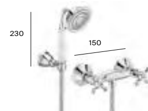
Twin-lever wall-mounted shower mixer with 1.5m flexible shower hose, handset and bracket
