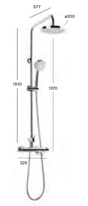
Wall-mounted thermostatic shower column Wall-mounted thermostatic shower column Wall-mounted thermostatic height adjustable shower column Wall-mounted thermostatic bath-shower column with retractable bath spout
