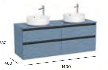
1400mm base unit and countertop with 4 soft-close drawers
