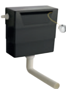
Universal Access Dual Flush Concealed Cistern Side Inlet, with Dual Flush Button H303 x W334 x D136mm BAYA102 £77.00
