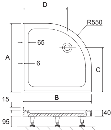
Quadrant upstand tray
