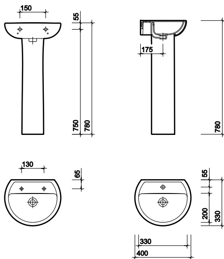
Alcona 400 x 330mm handrinse basin
