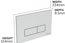
Oleas M2 Mechanical Dual Flushplate
