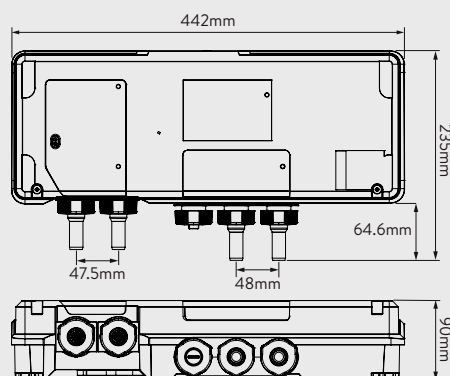
SMARTVALVE - GRAVITY PUMPED
