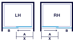
Sliding Door in Recess
