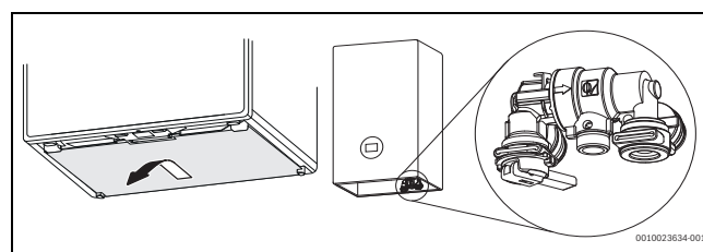
Fig. 3 Enable access to keyless filling link
