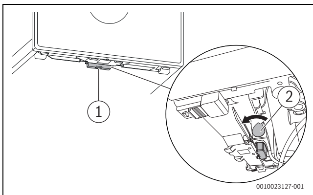
Fig. 8 Locking mechanism
