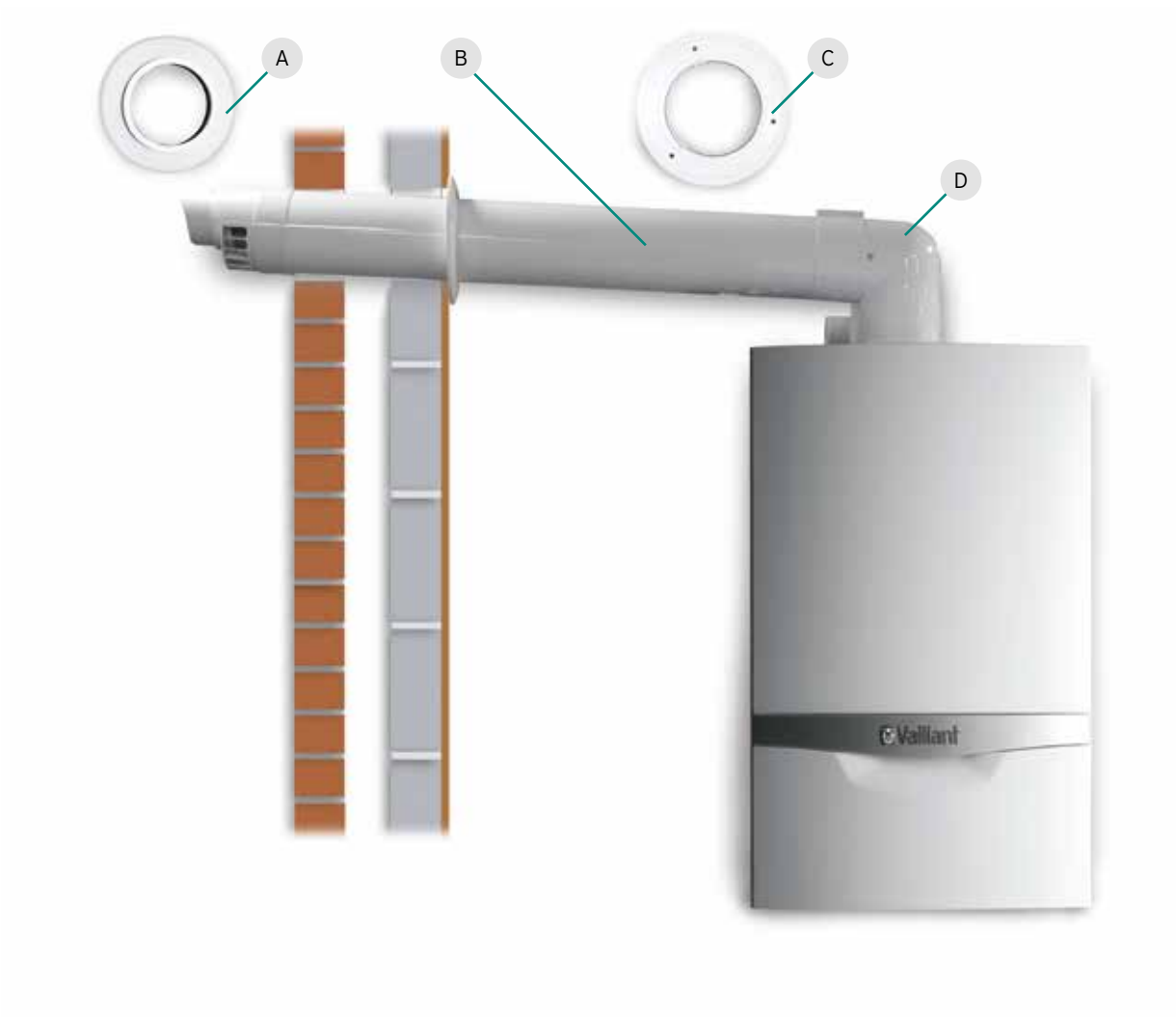
80/125mm concentric horizontal flue
