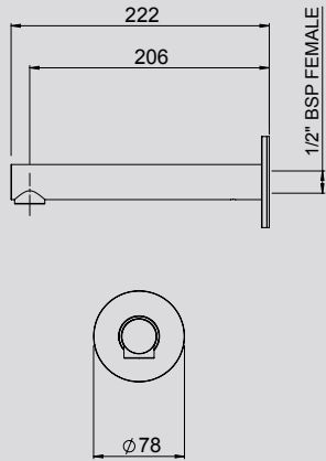
TŪROA WALL MOUNTED BATH SPOUT
