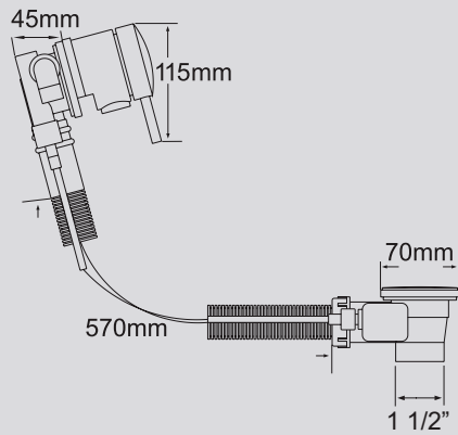
BATH FILL AND OVERFLOW
