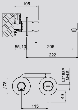
TŪROA WALL MOUNTED MIXER WITH SPOUT
