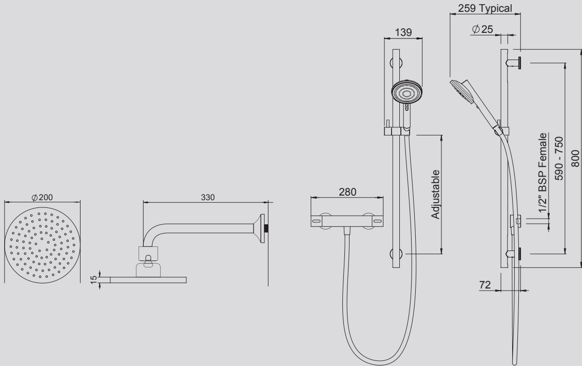
TŪROA OVERHEAD AND WALL ARM
